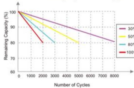
Different DOD Discharge Cycle Life Curve @1C
