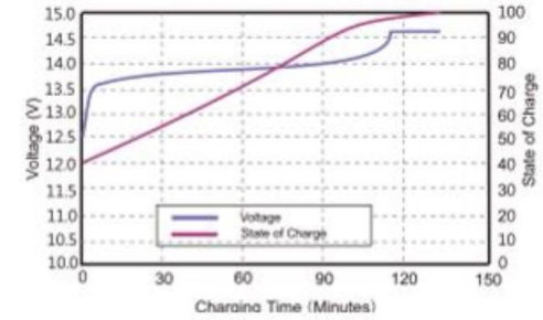
State of Charge Curve @0.5C 25°C
