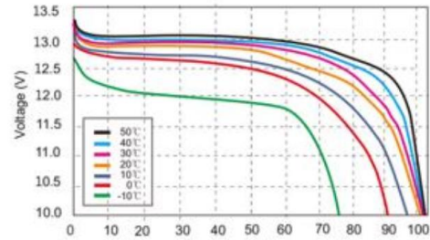
Different Temperature Discharge Curve @0.5C
